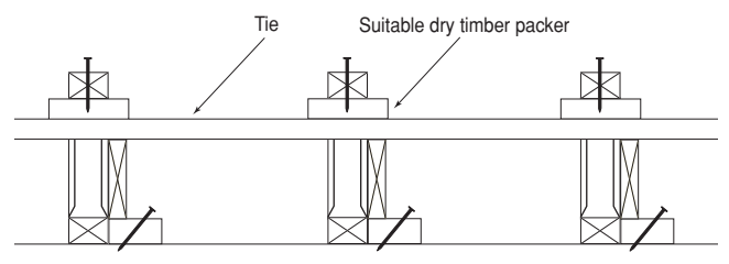
SECTION Y-Y
