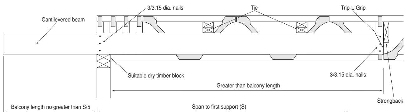
SECTION Y-Y
