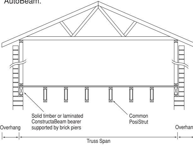
End wall - Single Storey
